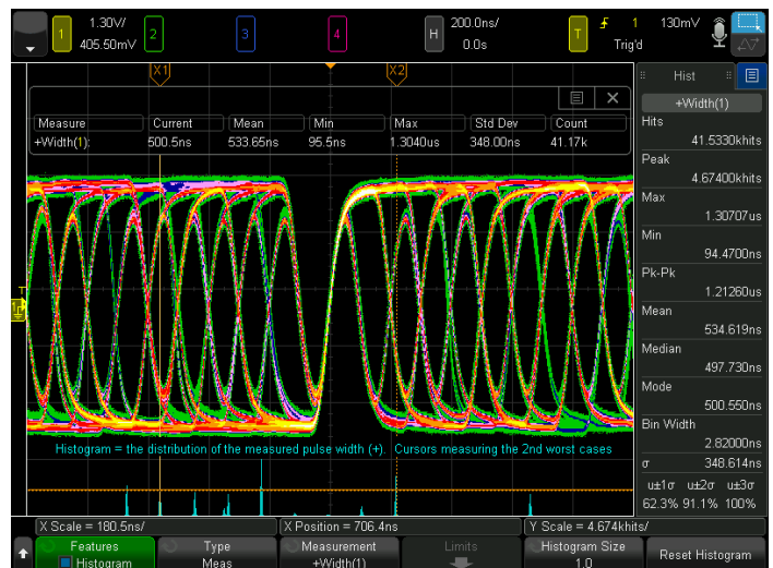
Figure 16b. Histogram plotting the results of the pulse width measurement.
